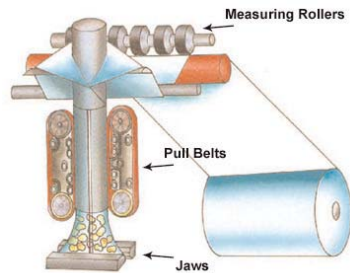
Hayssen's patented Measure, Form, Pull system is the fastest, production-proven way to package food.
