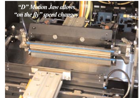
Ultima TR - Backseal Assembly
